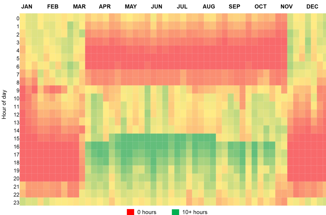
Figure 9. Resiliency across month and hour – 4-hour full load system.
