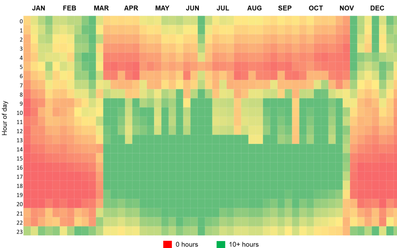
Figure 10. Resiliency across week and hour: 4-hour critical load system.
